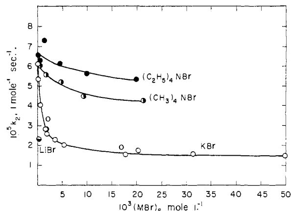
Fig. 1.—Rate constants at 0° for v = k_2(\text{RBr})(\text{MBr})_s .
